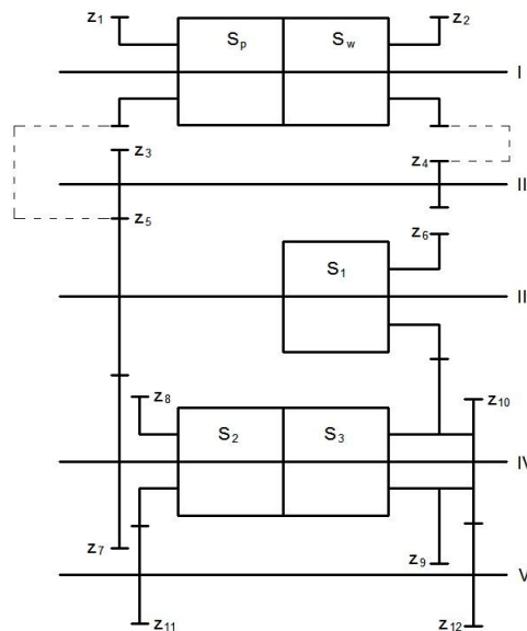
Fig.1 Kinematic scheme of a gearing in axial alignment:
