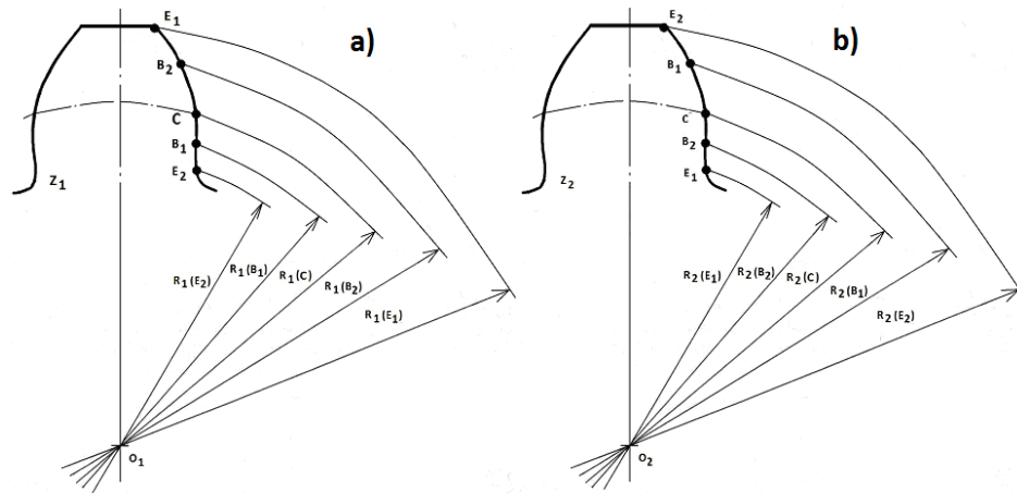
Fig. 5. Location of characteristic points: a) on the tooth of the drive gear, b) on the tooth of the driven gear
