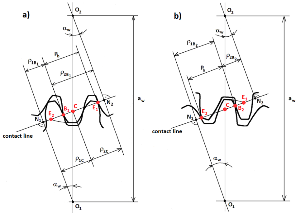
Fig.3 Toothed pair with the following tooth engagement area: a) B_1E_1 , b) B_2E_2
