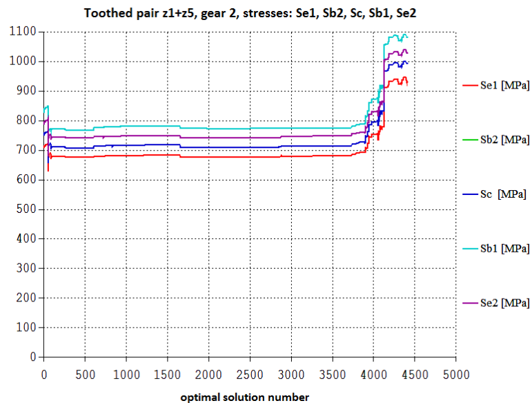
Fig. 8. Contact stresses in 5 characteristic points
